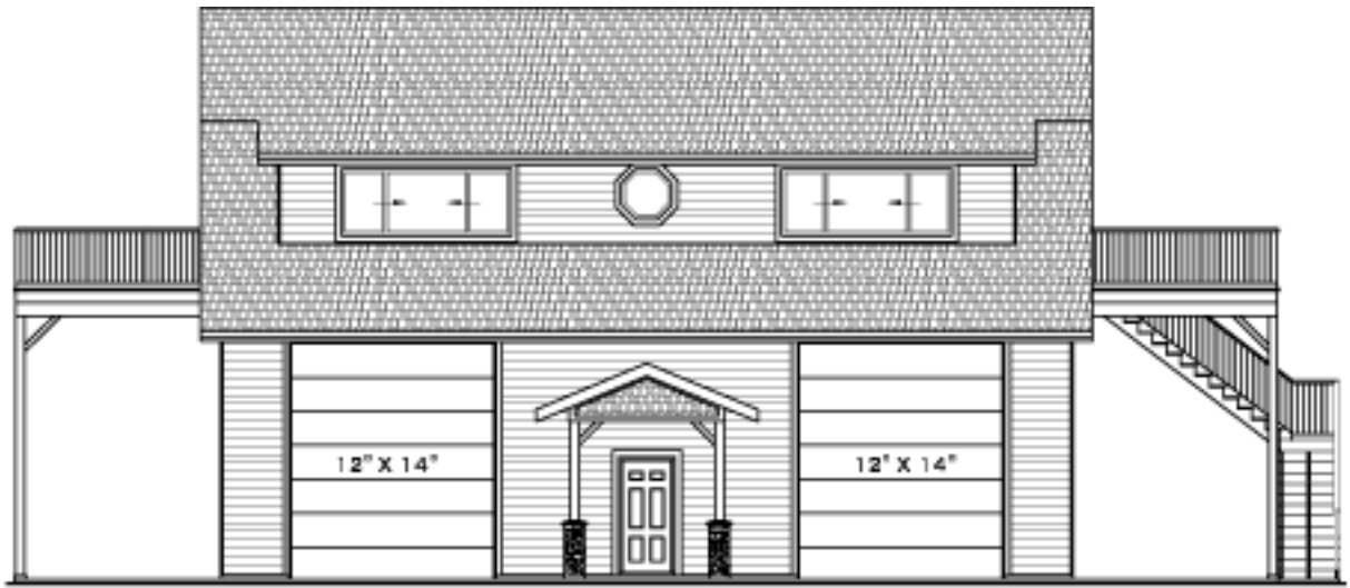
FRONT ELEVATION
